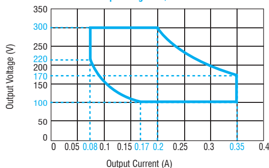
Output Range - 90/700
